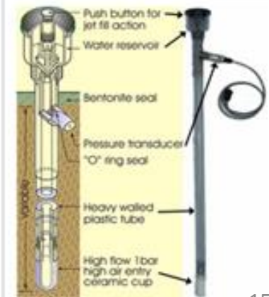
Tensiometer
